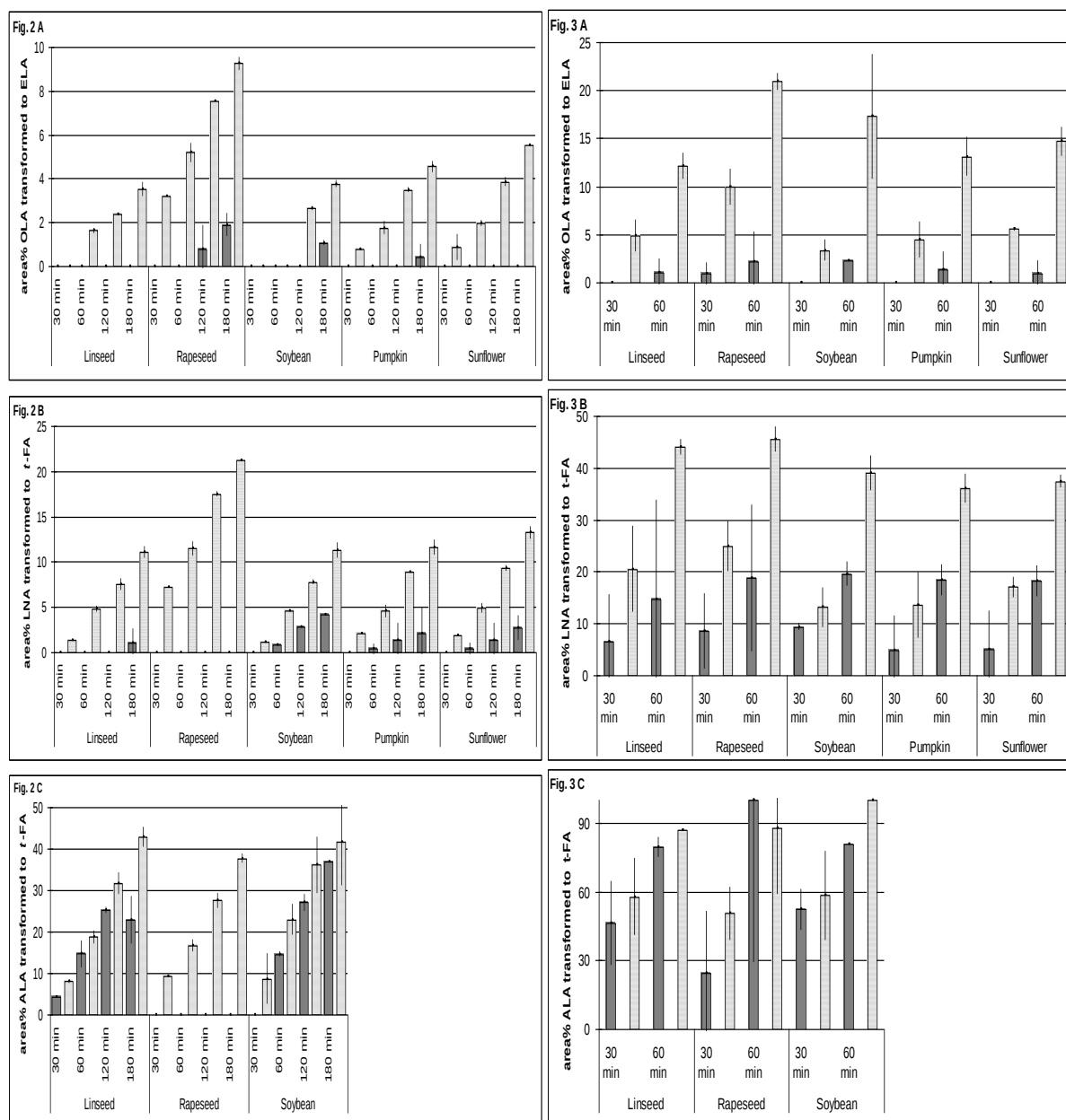
Fig. 2A-C Formation of trans -isomers=TI of oils and seeds (eic=OLA -, lino-leic=LNA- and alpha-linolenic-acid=ALA in area % of all isomers at 523 K,
