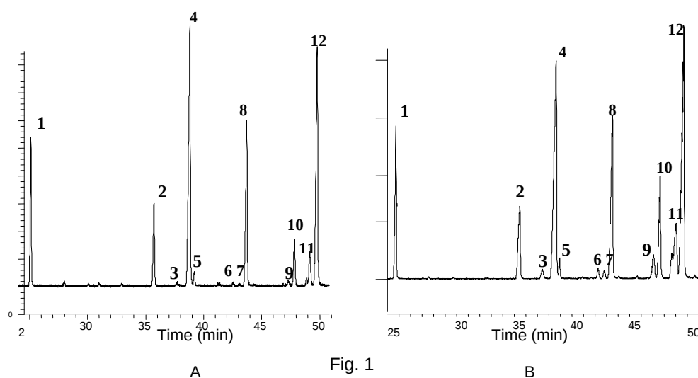
Fig. 1. GC/MS-chromatogram of linseed oil-methylesters (A from oil, B from seeds), heated 120 min/523 K. 1 = palmitate, 2 = stearate, 3 = elaidic acid, 4 = oleic acid, 5 = undefined fatty acid, 6 = cis-9, trans-12-linoleic acid, 7 = trans-9, cis-12-linoleic acid, 8 = all-cis-linolenic acid, 9 = 2xtrans, 1xcis-linolenic acid, 10 = cis-9, cis-12, trans-15-linolenic acid, 11 = cis-9, trans-12, cis-15- and trans-9, cis-12, cis-15-linolenic acid, 12 = all-cis-linolenic acid
