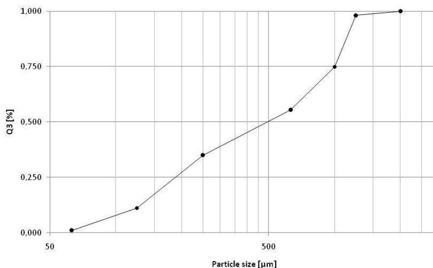
Fig. 1. Cumulative particle size distribution of dairy cow feed.
