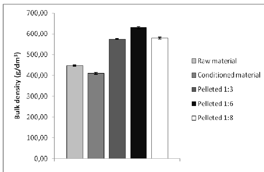
Fig. 5. Bulk density of material during processing Results are given as mean \pm Standard deviation
