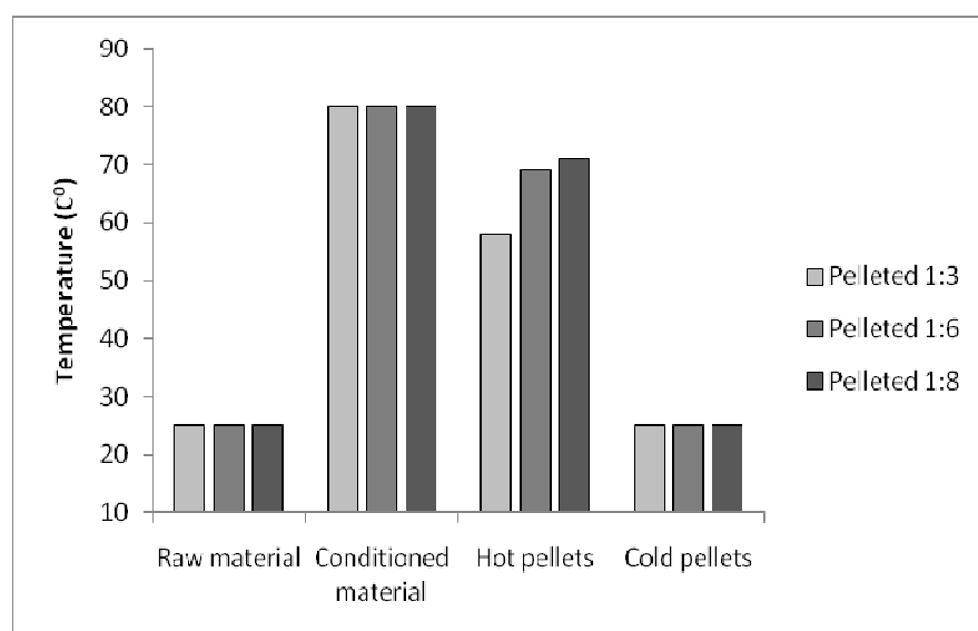
Fig. 4. Temperature of material during processing
