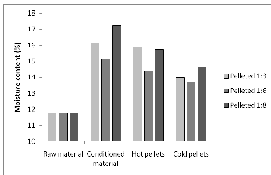
Fig. 3. Moisture content of material during processing
