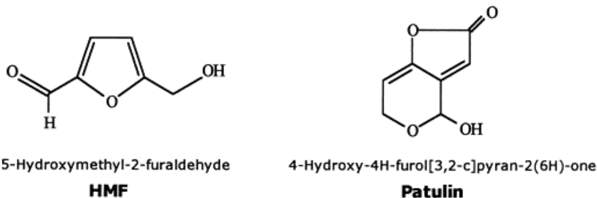
Figure 1. Chemical structures of 5-HMF and patulin
